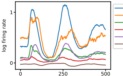
Trace of LM population firing rate component
